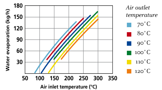
VSD-50 co-current atomization
