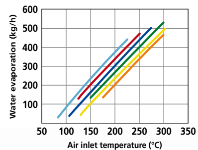
VSD-80 co-current atomization
