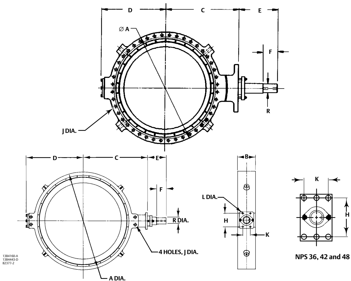
Figure 4. Dimensions Wafer and Single Flange Style CL150 (also see table 9)
