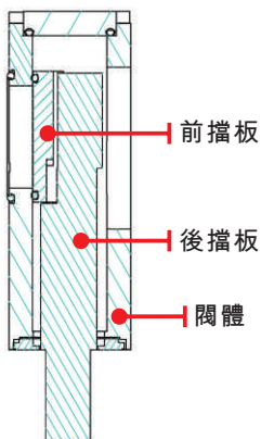
Closed position
