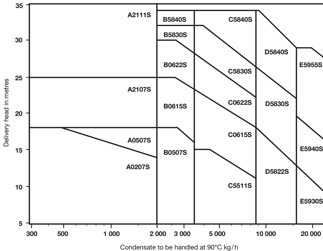
Single pump sizing chart at 90°C
